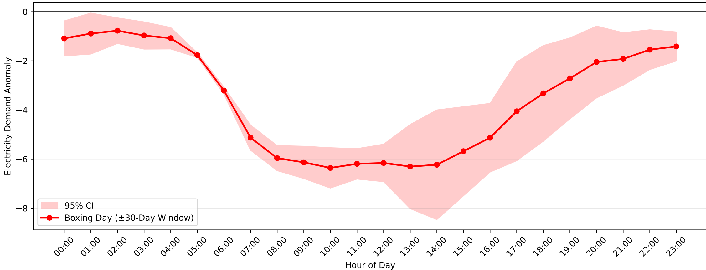
Bankstown Demand Anomaly: Boxing Day (2011-2012, \pm 30 -Day Window)
