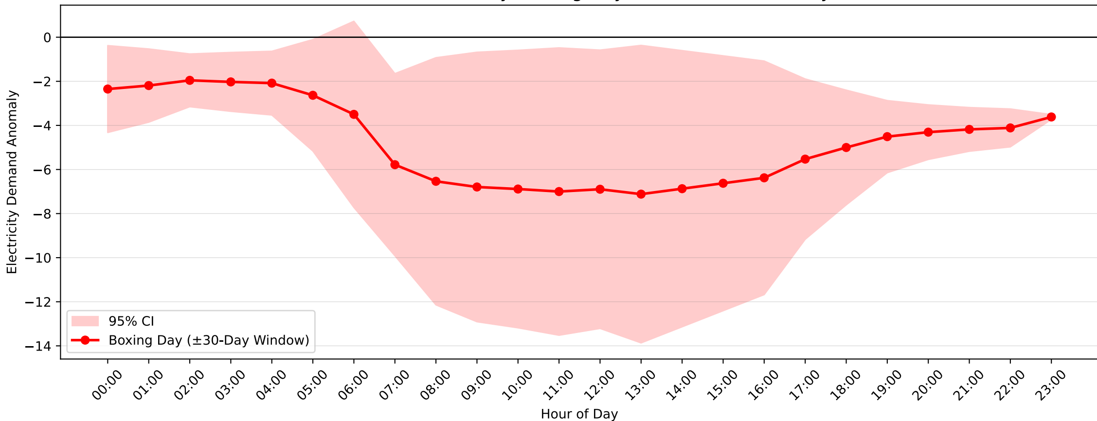
Bankstown Demand Anomaly: Boxing Day (2013–2014, \pm 30 -Day Window)
