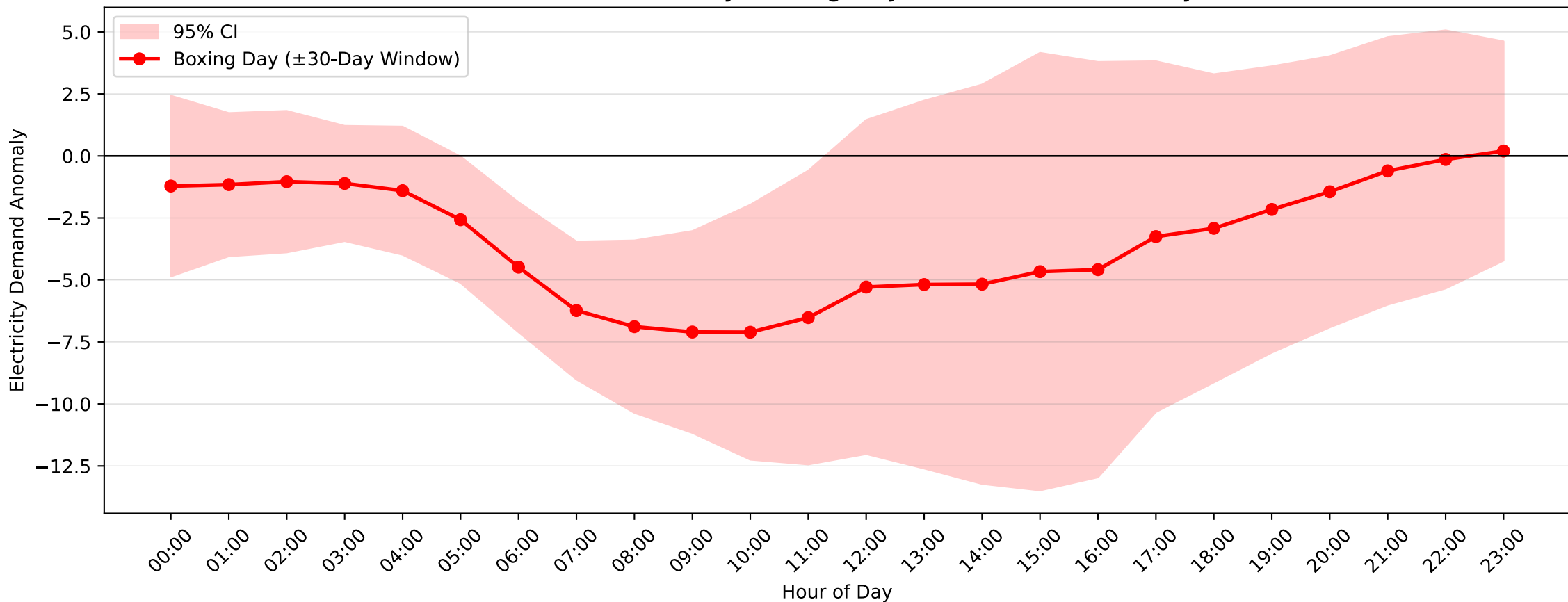
Bankstown Demand Anomaly: Boxing Day (2015–2016, \pm 30 -Day Window)
